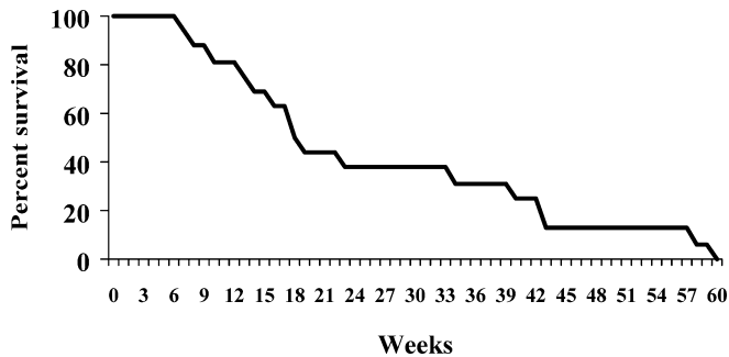
Fig. 2 Kaplan-Meier curve showing overall survival
